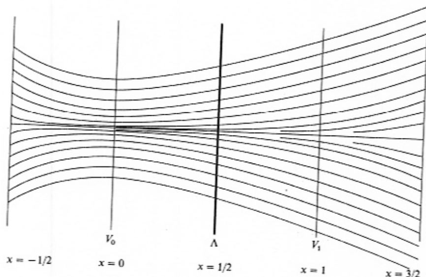
FIGURE 6. Overpinched holonomy
