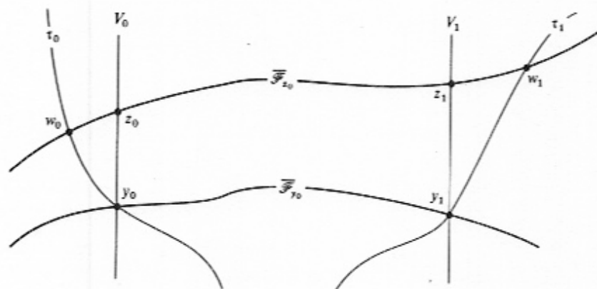
FIGURE 4. Comparing the holonomy in T_p M between vertical transversals and between transversals of coslope \leq L
