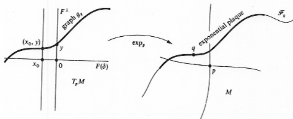
FIGURE 3. Plaques in T_p M and M
