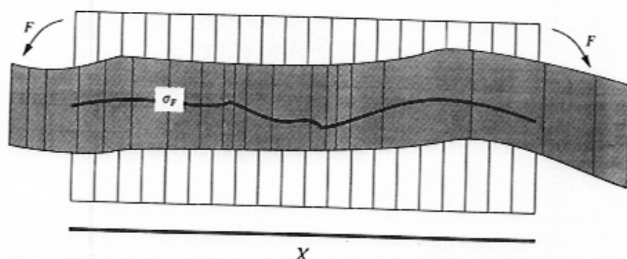
FIGURE 2. A fiber contraction and its invariant section
