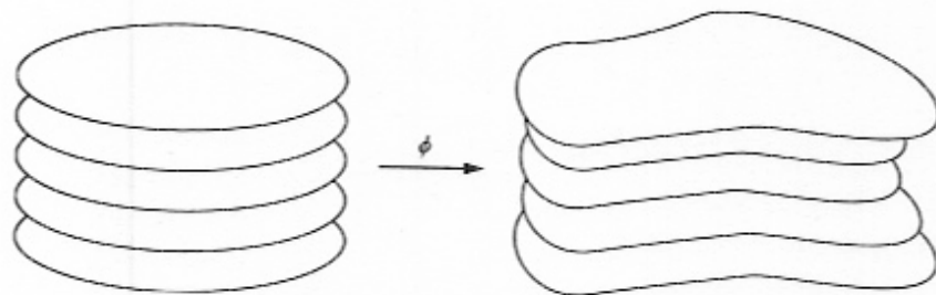
FIGURE 8. The foliation chart \phi
