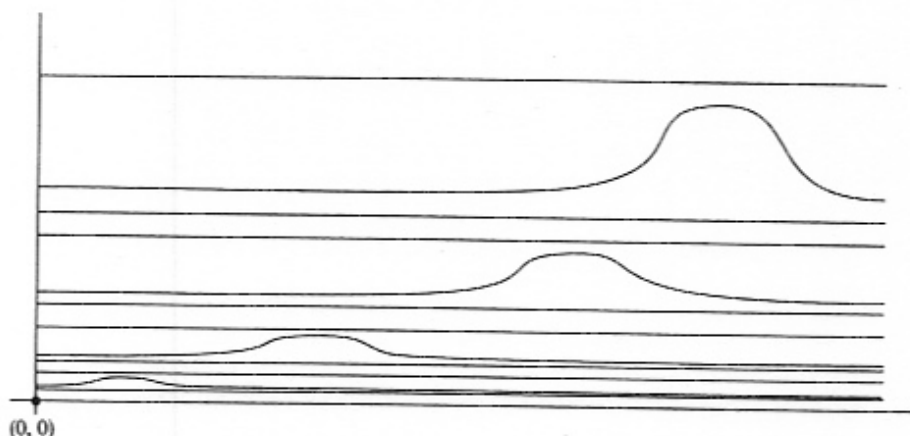
FIGURE 9. A foliation whose leaves are uniformly C^\infty and whose holonomy is C^\infty , but which does not have uniformly C^1 holonomy and is therefore not a C^1 foliation
