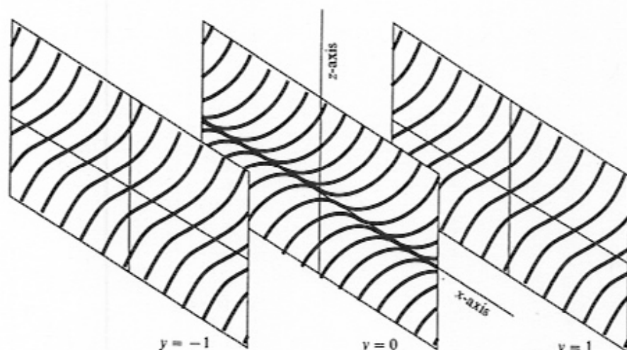
FIGURE 10. The trace of a nonunique foliation on three (x, z) -planes
