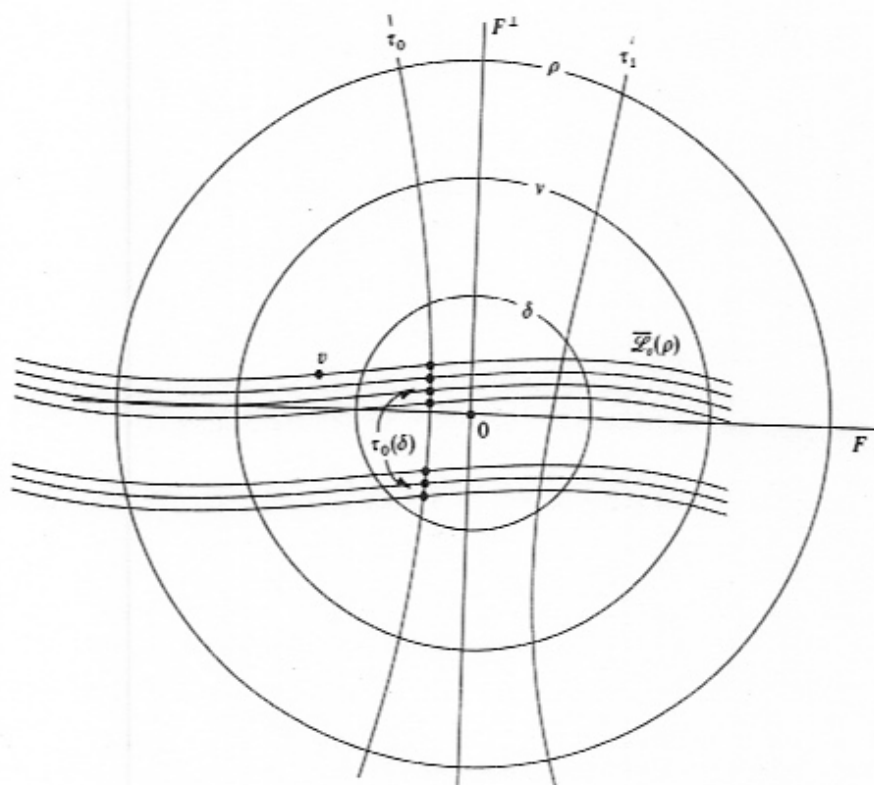
FIGURE 5. The local holonomy along \bar{\mathcal{L}}
